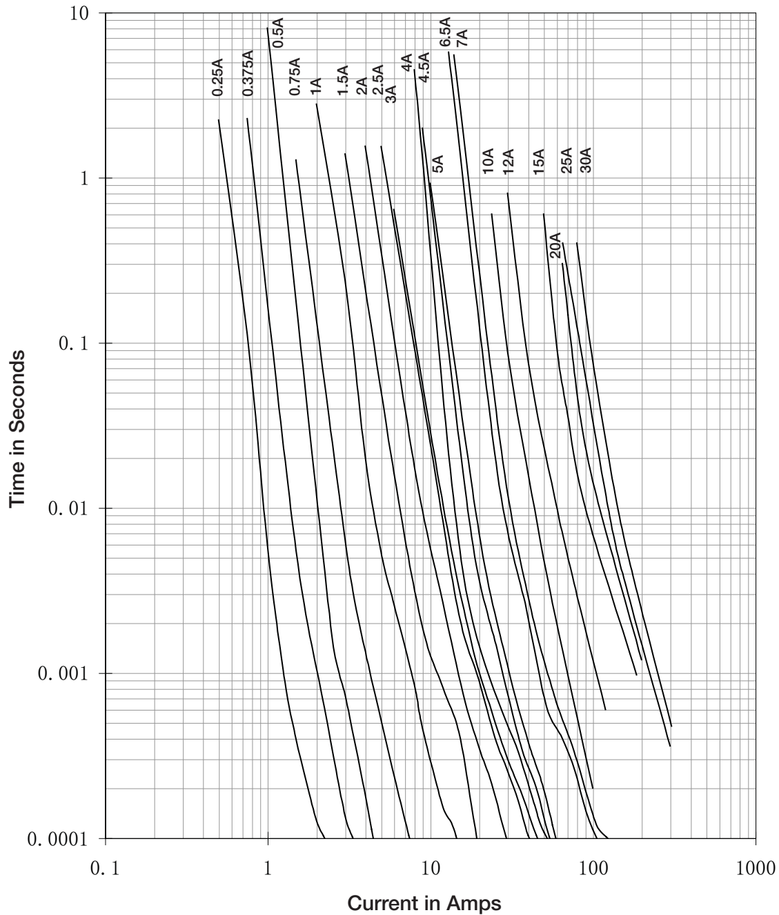
Time-Current Curve
