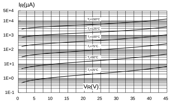
Figure 6: Reverse leakage current versus reverse voltage applied (typical values)
