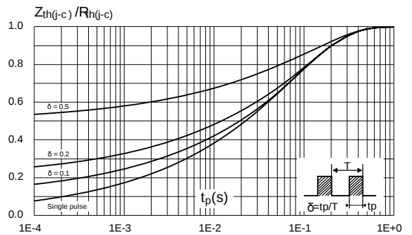
Figure 4: Relative variation of thermal impedance junction to case versus pulse duration (TO-220AC and D 2 PAK)
