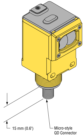
Micro-style Quick-disconnect
