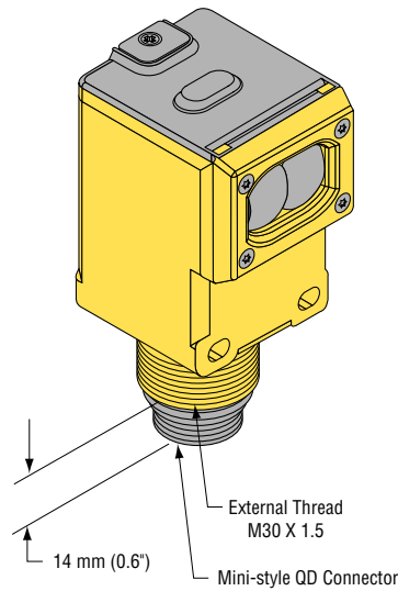
Mini-style Quick-disconnect
