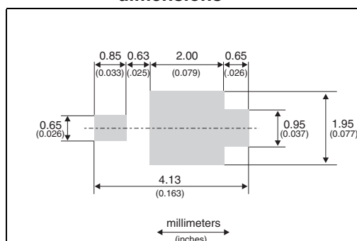
Figure 11. STmite flat footprint dimensions
