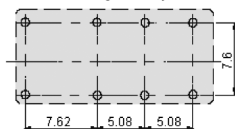
Mounting Hole Layout
