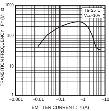
Fig.7 Transition frequency
