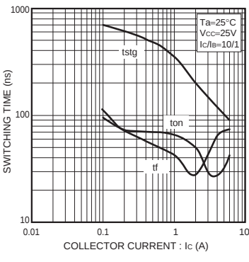
Fig.9 Switching Time
