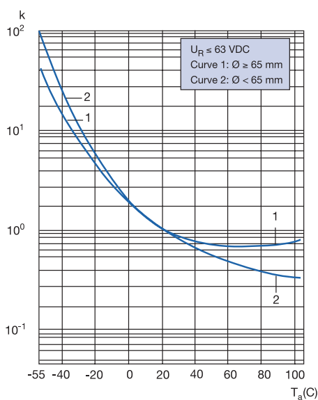
ESR as a function of ambient temperature ( T_a ) at f = 100 kHz. k = R_{ESR}(T_a)/R_{ESR}(20°C)
