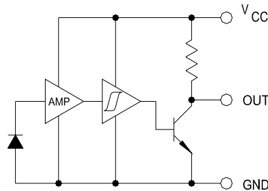
OPB617/627/667N Inverted 10K Pull-Up
