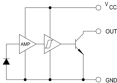
OPB618/628/668N Inverted Open-Collector
