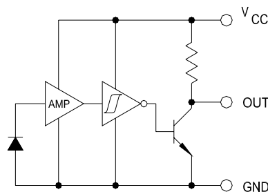
OPB617/627/667N Inverted 10K Pull-Up
