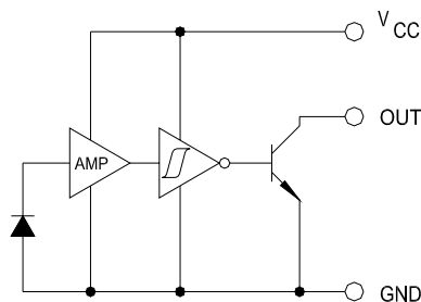
OPB618/628/668N Inverted Open-Collector
