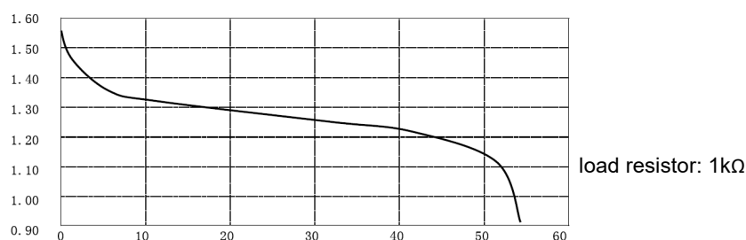
Typical Discharge Characteristics at 20°C
