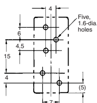
Terminal Arrangement (Bottom View)
