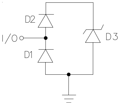
Figure 1 - RClamp0504P Spice Model
