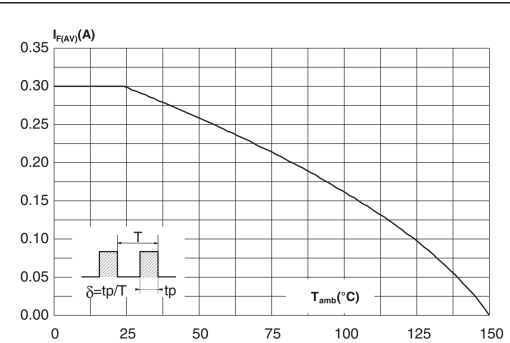
Figure 2. Average forward current versus ambient temperature ( \delta = 1 )
