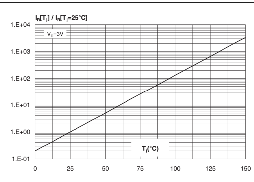
Figure 4. Reverse leakage current versus junction temperature
