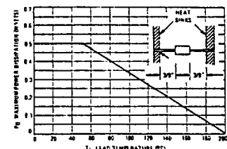
Figure 2 POWER DERATING
