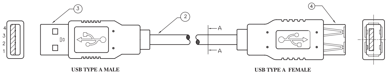
USB TYPE A MALE
