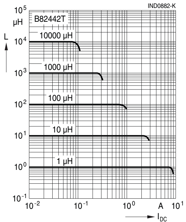
Inductance L versus DC load current I_{\text{DC}} measured with LCR meter Agilent 4285A, typical values at +20 °C
