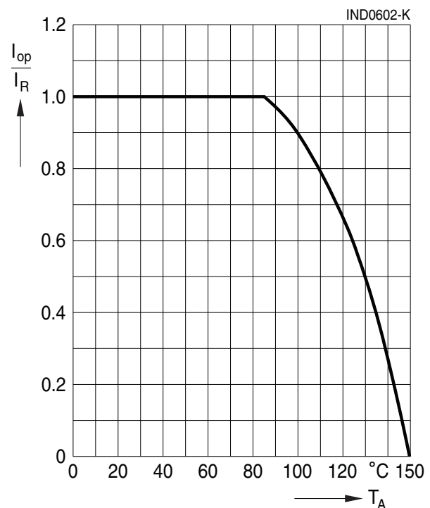
Current derating I_{\text{op}}/I_{\text{R}} versus ambient temperature T_{\text{A}} (rated temperature T_{\text{R}} = +85 °C)
