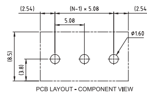
PCB LAYOUT - COMPONENT VIEW
