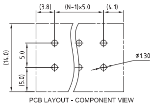
PCB LAYOUT - COMPONENT VIEW
