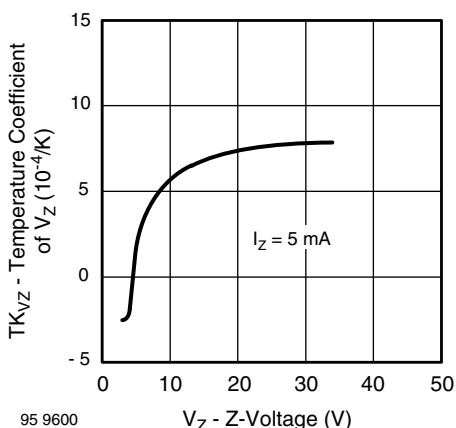
Fig. 2 - Typical Temperature Coefficient of V_Z vs. Z-Voltage
