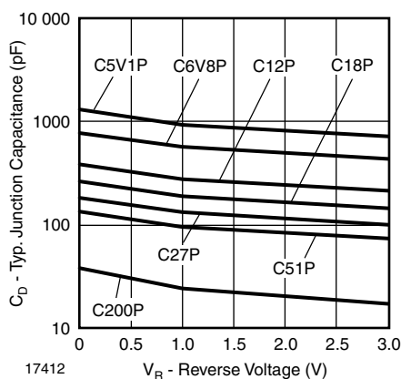
Figure 2. Typ. Diode Capacitance vs. Reverse Voltage
