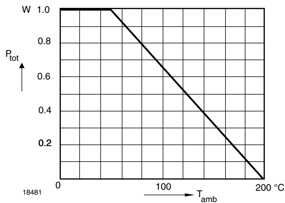
Fig. 1 - Admissible Power Dissipation vs. Ambient Temperature
