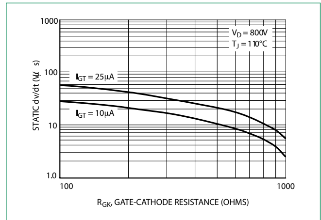
Figure 12. Exponential Static dv/dt vs Gate–Cathode Resistance and Gate Trigger Current Sensitivity
