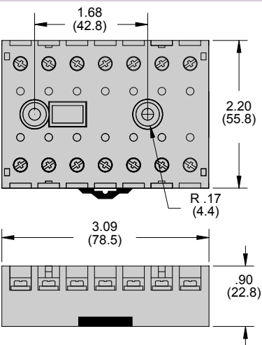
14 Pin Socket - 33377D
