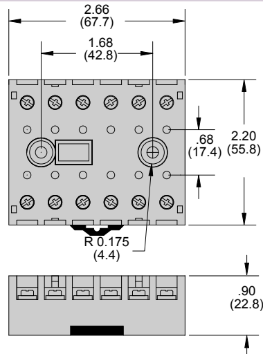
12 Pin Socket - 27390D
