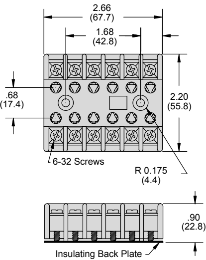
12 Pin Socket - 27390
