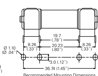
0106 0001 Device Dimensions
