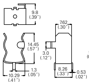
0106 0001 Device Dimensions
