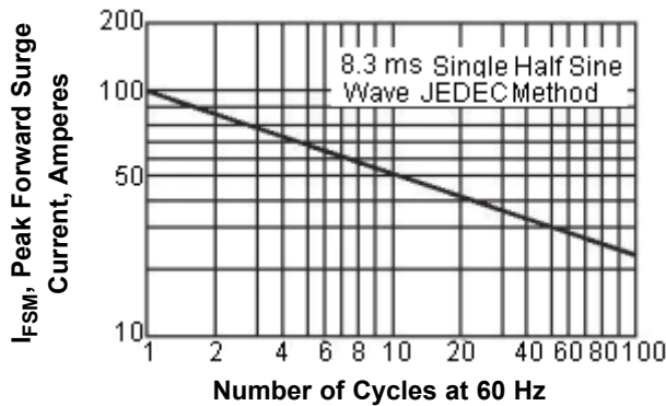
Maximum Non-Repetitive Forward Surge Current Unidirectional Only
