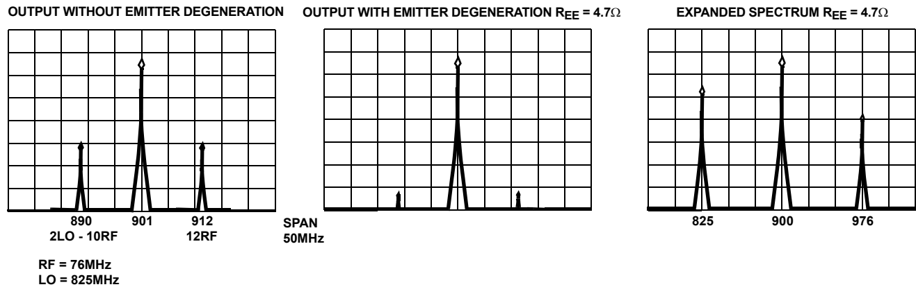
FIGURE 13. TYPICAL SPECTRUM PERFORMANCE OF UP CONVERTER
