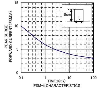
IFSM-t CHARACTERISTICS
