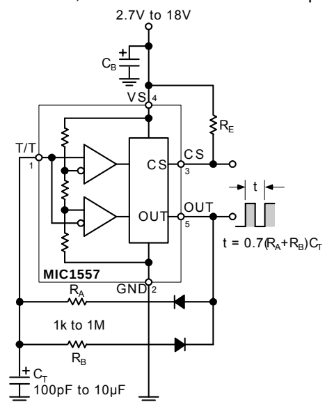
Figure 2. Oscillator Diagram
