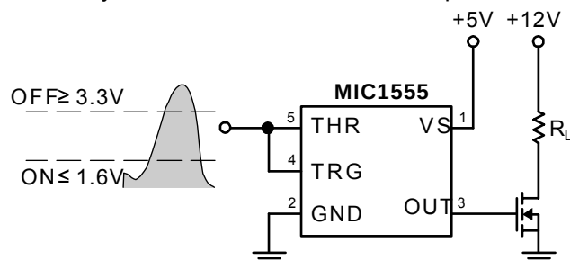
Figure 7. Schmitt Trigger
