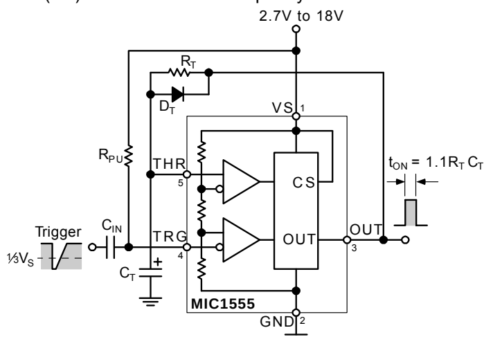
Figure 1. One-Shot Diagram
