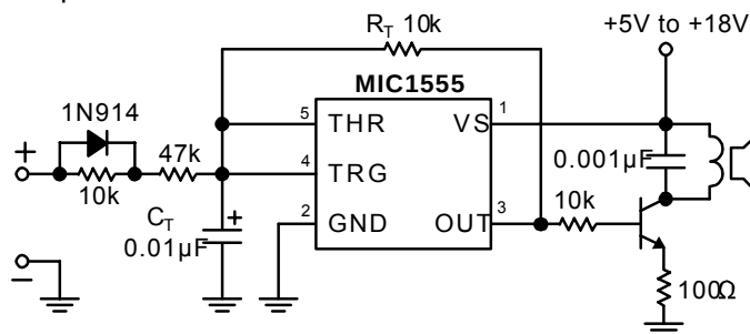
Figure 9. Audible Voltmeter
