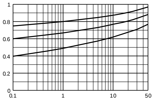
Figure 3. Base-Emitter Saturation Voltage vs Collector Current
