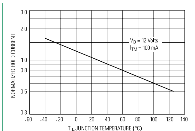
Figure 8. Holding Current
