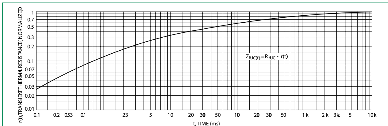
Figure 5. Thermal Response
