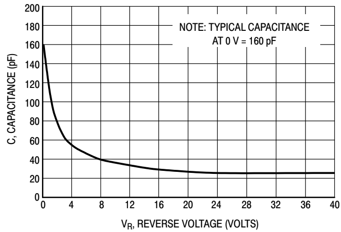
Figure 3. Typical Capacitance
