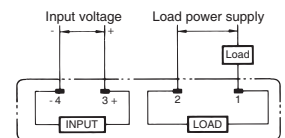
Terminal Arrangement (BOTTOM VIEW)
