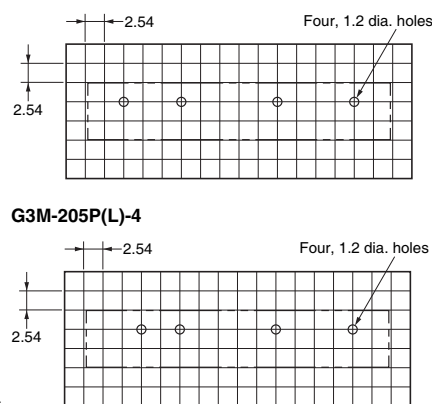
PCB Dimensions (BOTTOM VIEW) G3M-205P(L)
