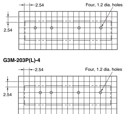
PCB Dimensions (BOTTOM VIEW) G3M-203P(L)
