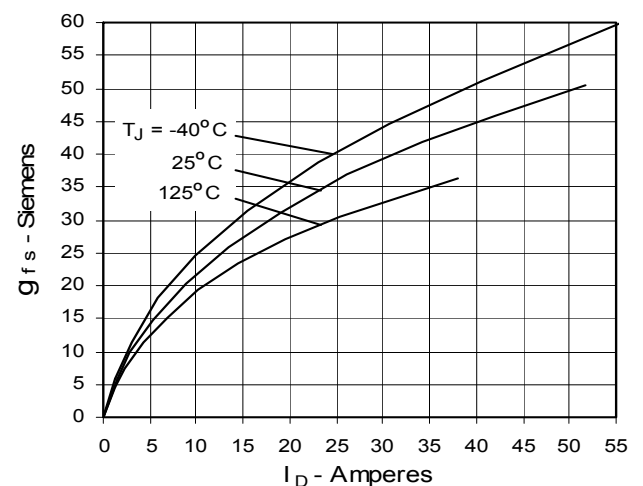
Fig. 8. Transconductance
