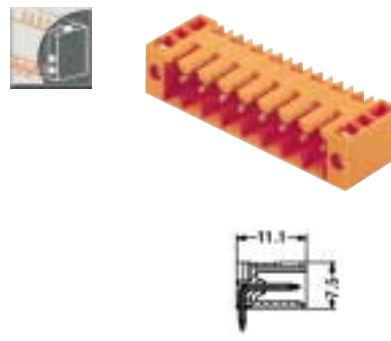
Pin headers SL 3.5/90F
