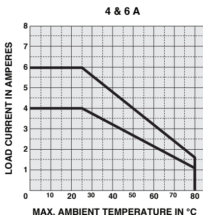
Load Current vs Ambient Temperature (100% Duty Cycle)
