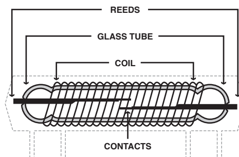
Typical Reed Relay
