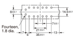
Mounting Hole Dimensions
