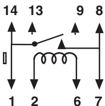
Figure G SPST-NO Without diode
