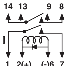
Figure L DPST-NO With diode
