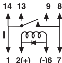
Figure H SPST-NO With diode
