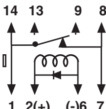
Figure J SPST-NC With diode
