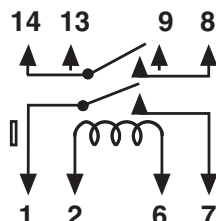
Figure K DPST-NO Without diode
