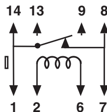
Figure I SPST-NC Without diode
