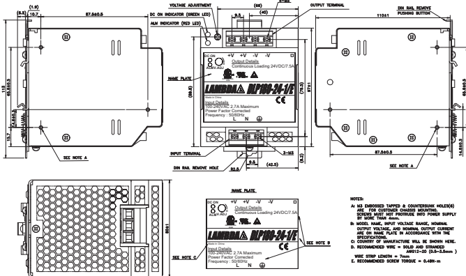
DLP180 Outline
