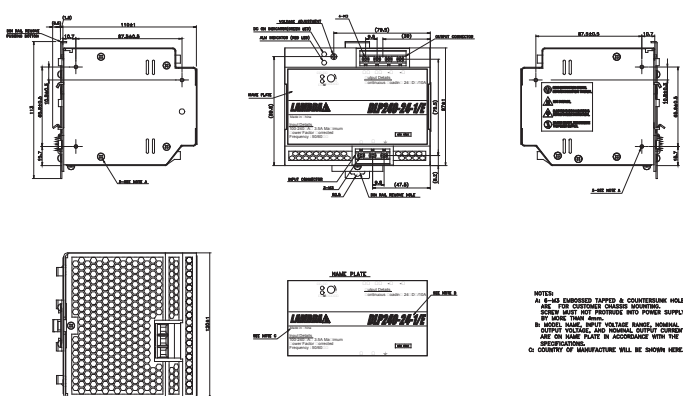
DLP240 Outline
