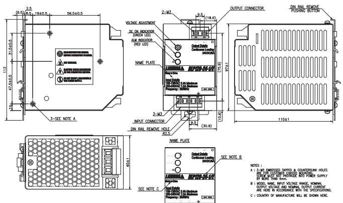
DLP100/120 Outline
