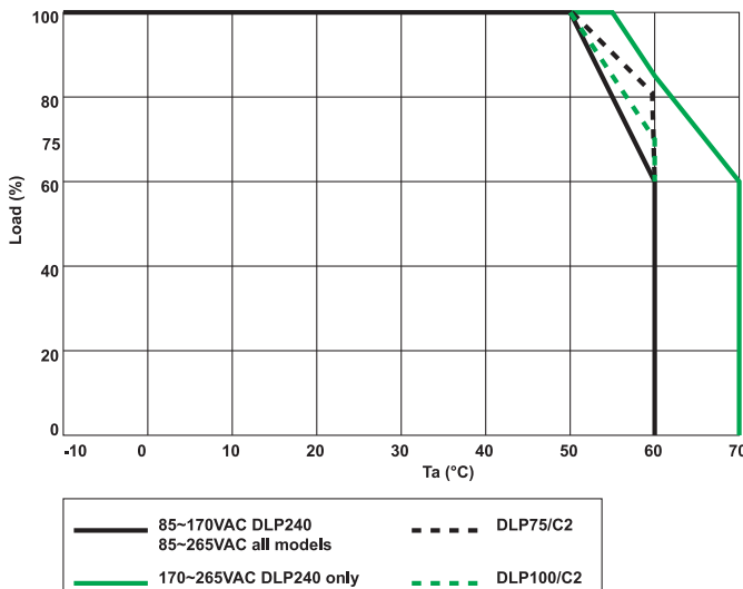
Derating Curve
