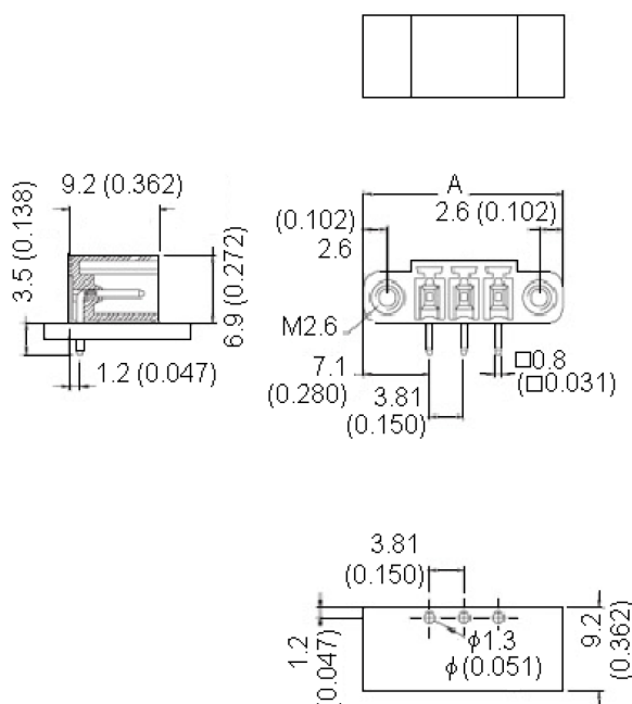
Dimensions : Millimetres (Inches) PCB Layout
