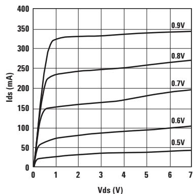
Figure 6. Typical IV Curve.
