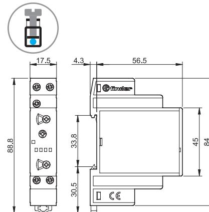
80.71 Screw terminal
