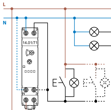
4 wire connection
