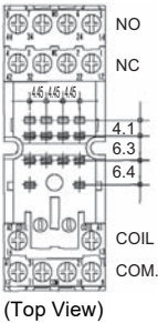
Terminal arrangement/ Internal connections/ mounting holes
