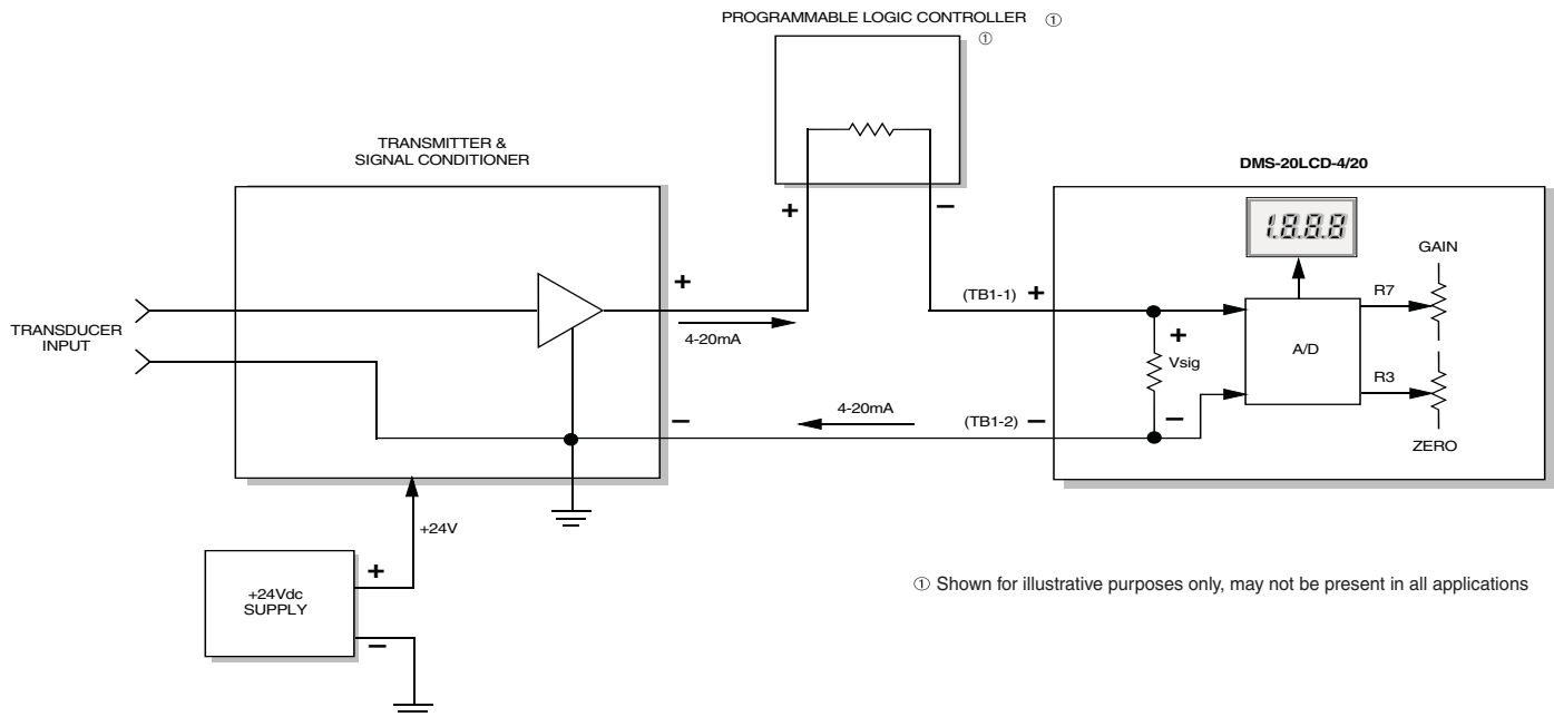
Figure 2. Typical DMS-20LCD-4/20 Connection Diagram
