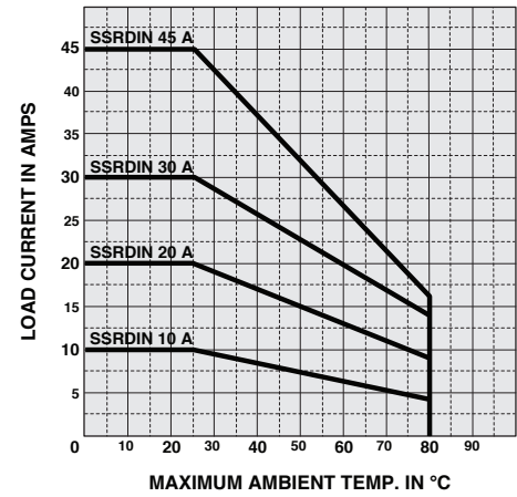
Load Current vs Ambient Temperature (100% Duty Cycle)
