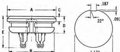
78-S8 socket and retainer ring
