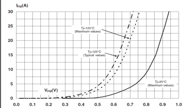
Figure 7: Forward voltage drop versus forward current (per diode, low level)
