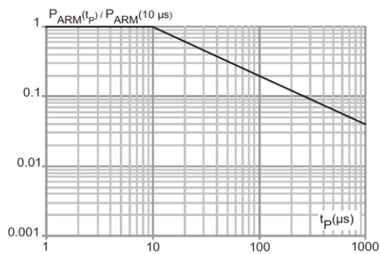
Figure 3: Normalized avalanche power derating versus pulse duration ( T_j = 125^\circ\text{C} )
