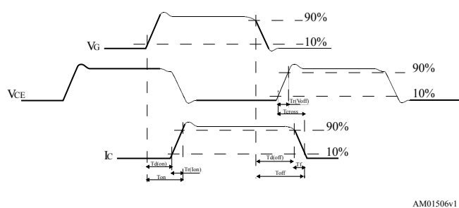
Figure 19. Switching waveform
