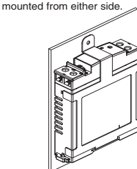
Face-up mounting with S82Y-VS30P
