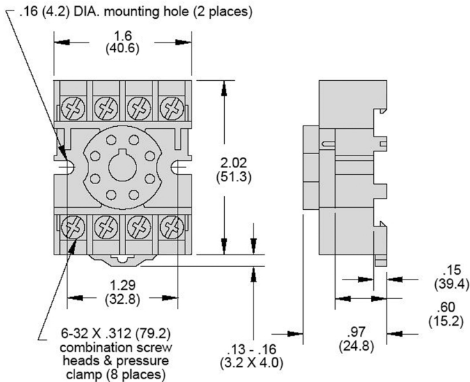
8 Pin Socket
